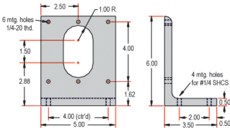
5.00" Z-Axis Adapter Plate (#54-380)
