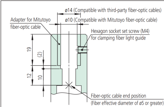
Detail of fiber mount
