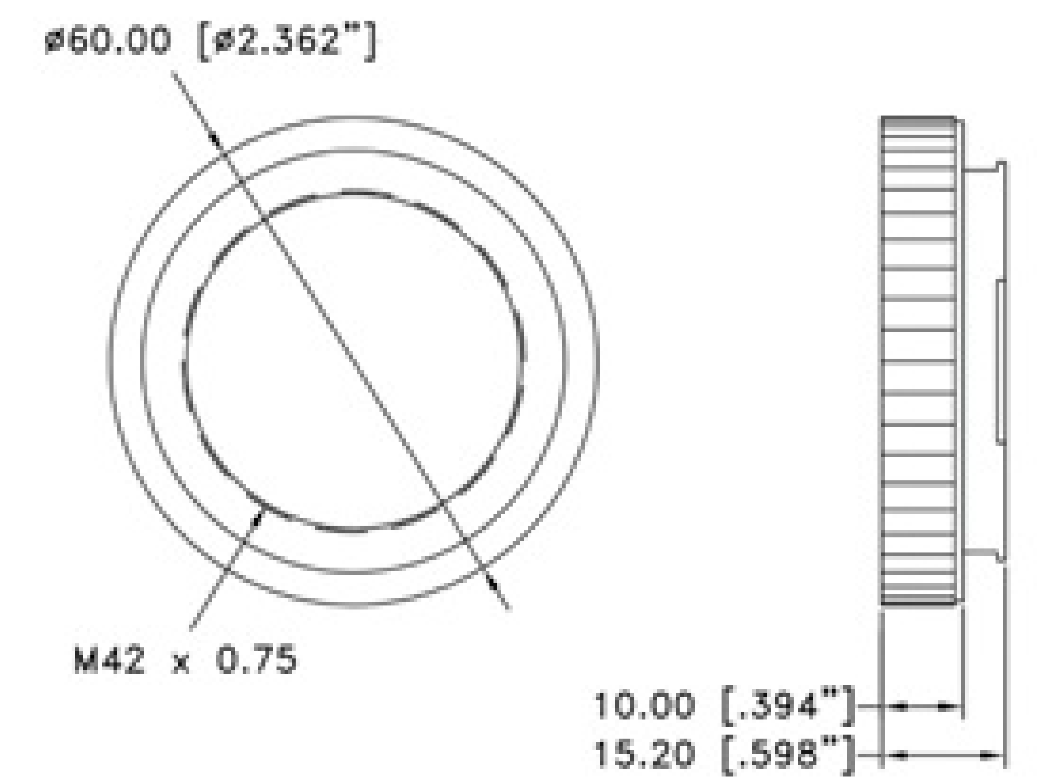
#16-139: T-Mount (M42) to Sony A Mount
