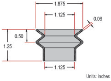
Style B) 1.125" Rubber Eyeguard
