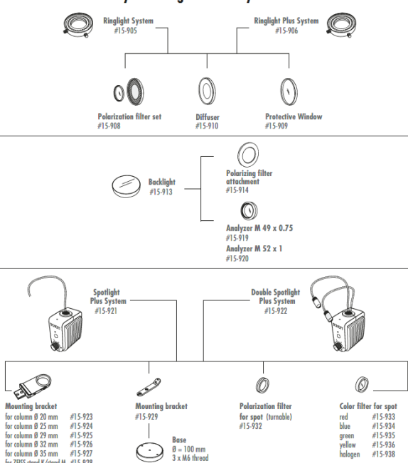
System Diagram for EasyLED Series
