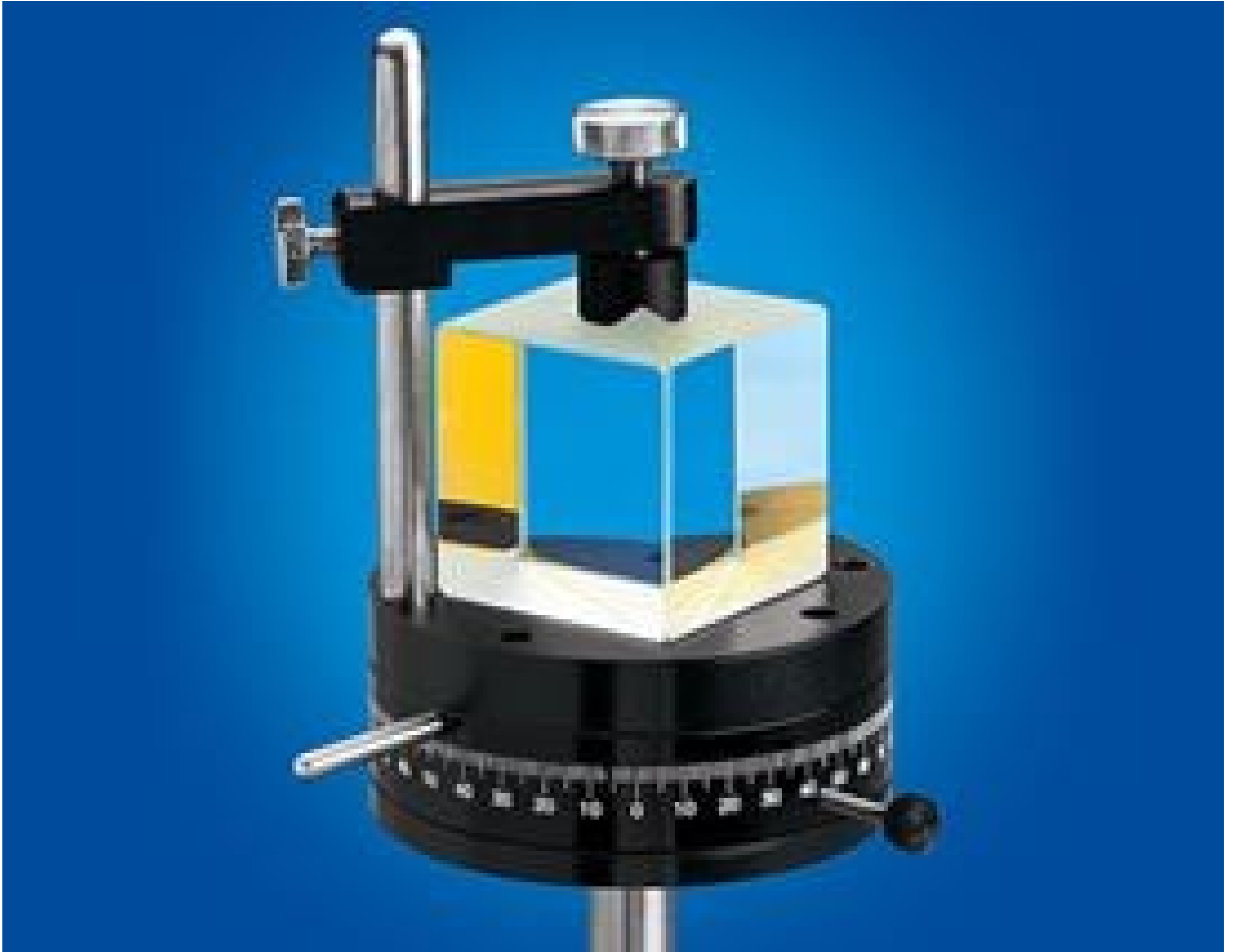
#53-027 + Cube Beamsplitter
