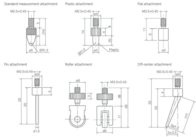
PID4485_Measurement_Probes
