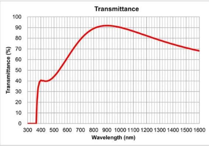
LCPLN20XIR Transmission Graph
