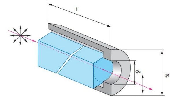
Glan-Taylor Polarizers
