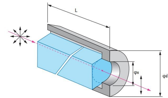
Glan-Taylor Polarizers
