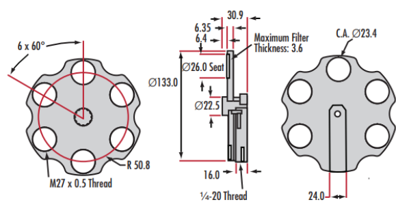
6-Position Filter Wheel Assembly
