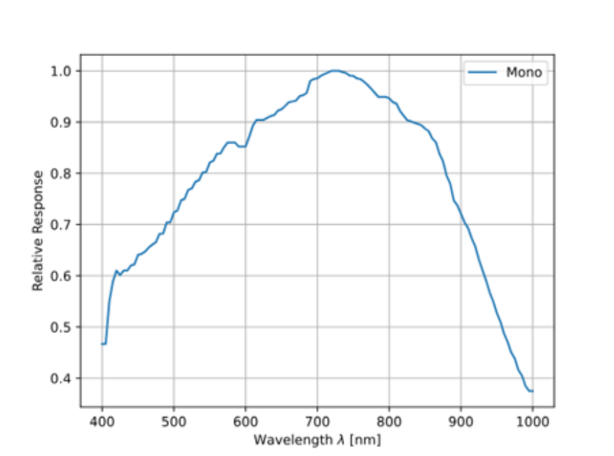
IMX676 Sensor QE Curve
