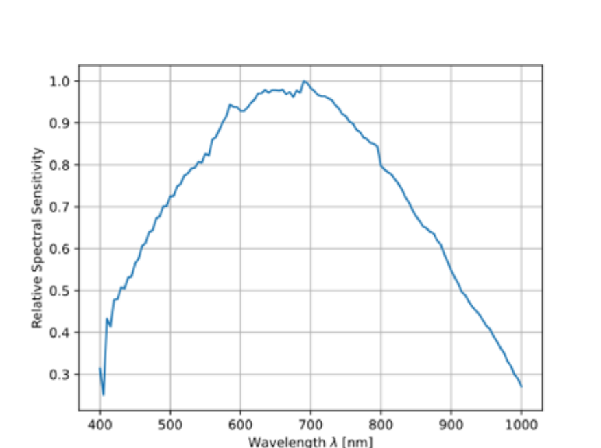
IMX900 Sensor QE Curve
