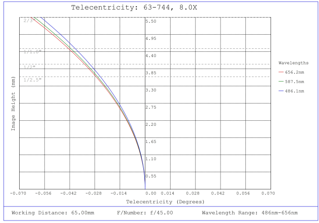
#63-744, 8X, 65mm WD CompactTL™ Telecentric Lens, Telecentricity Plot
