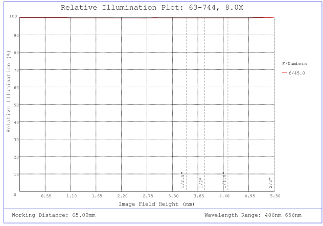
#63-744, 8X, 65mm WD CompactTL™ Telecentric Lens, Relative Illumination Plot
