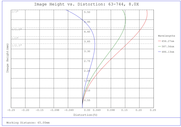
#63-744, 8X, 65mm WD CompactTL™ Telecentric Lens, Distortion Plot
