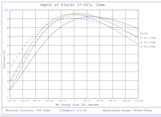
#37-523, 12mm FL, Liquid Lens M12 Lens, Depth of Field Plot, 500mm Working Distance, f2.4
