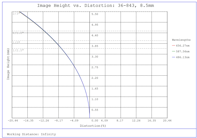
#36-843, 8.5mm, f/8 Cr Series Fixed Focal Length Lens, Distortion Plot
