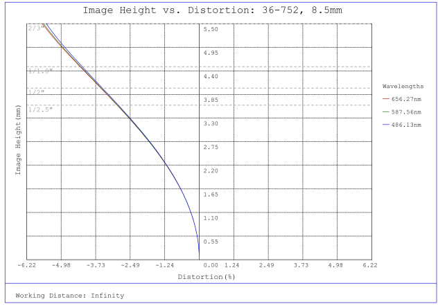
#36-752, 8.5mm f/8, 75mm-∞ Primary WD, HRi Series Fixed Focal Length Lens, Distortion Plot
