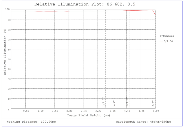
#86-602, 8.5mm, f/4 Ci Series Fixed Focal Length Lens, Relative Illumination Plot
