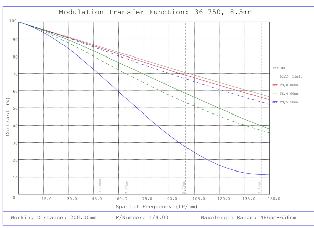
#36-750, 8.5mm f/4, 75mm-∞ Primary WD, HRi Series Fixed Focal Length Lens, Modulated Transfer Function (MTF) Plot, 200mm Working Distance, f4
