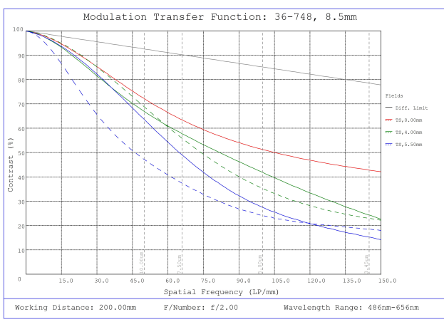
#36-748, 8.5mm f/2, 75mm-∞ Primary WD, HRi Series Fixed Focal Length Lens, Modulated Transfer Function (MTF) Plot, 200mm Working Distance, f2
