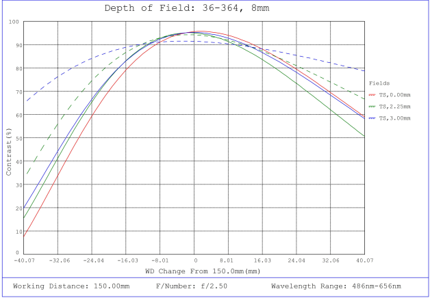
#36-364, 8.0mm FL f/2.5, Rugged Blue Series M12 Lens, Depth of Field Plot, 150mm Working Distance, f2.5
