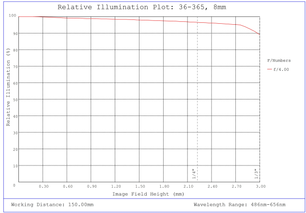
#36-365, 8.0mm FL f/4 Rugged Blue Series M12 Lens, Relative Illumination Plot
