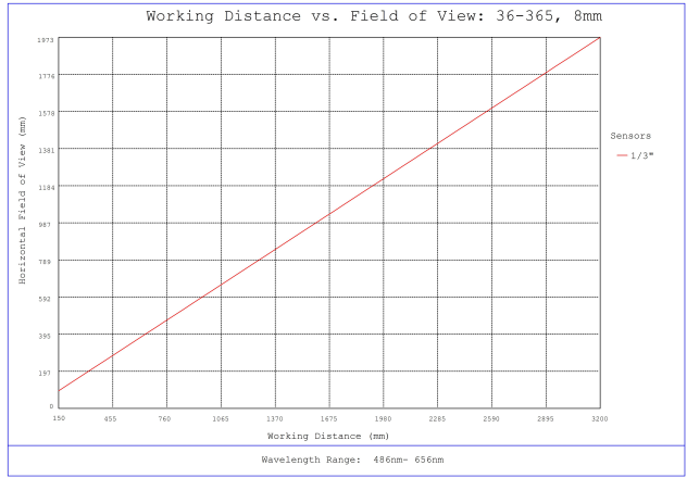
#36-365, 8.0mm FL f/4 Rugged Blue Series M12 Lens, Working Distance versus Field of View Plot
