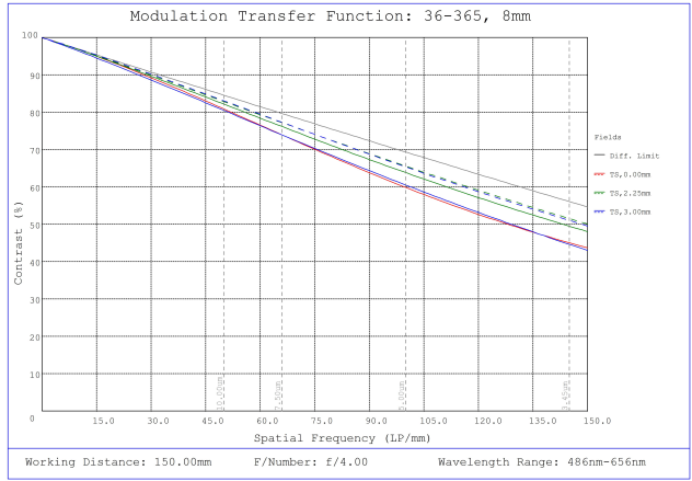
#36-365, 8.0mm FL f/4 Rugged Blue Series M12 Lens, Modulated Transfer Function (MTF) Plot, 150mm Working Distance, f4
