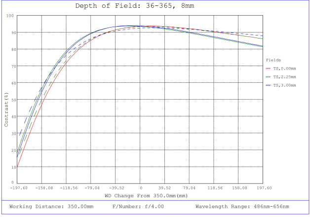
#36-365, 8.0mm FL f/4 Rugged Blue Series M12 Lens, Depth of Field Plot, 350mm Working Distance, f4
