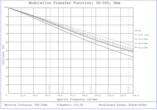
#36-365, 8.0mm FL f/4 Rugged Blue Series M12 Lens, Modulated Transfer Function (MTF) Plot, 350mm Working Distance, f4
