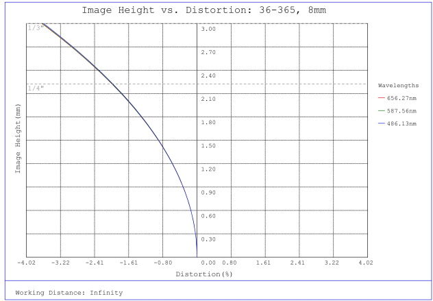
#36-365, 8.0mm FL f/4 Rugged Blue Series M12 Lens, Distortion Plot
