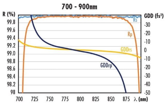
Ultrafast Ti:Sapphire Laser Mirror Reflection Curve
