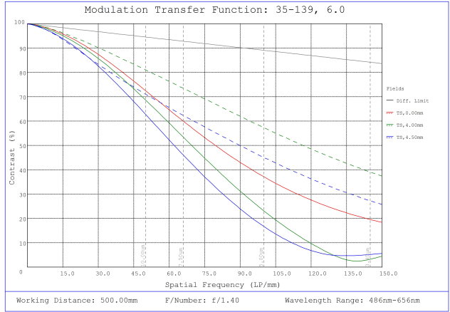
#35-139, 6mm, f/1.4 Cr Series Fixed Focal Length Lens, Modulated Transfer Function (MTF) Plot, 500mm Working Distance, f1.4
