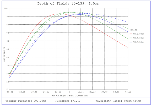
#35-139, 6mm, f/1.4 Cr Series Fixed Focal Length Lens, Depth of Field Plot, 200mm Working Distance, f1.4
