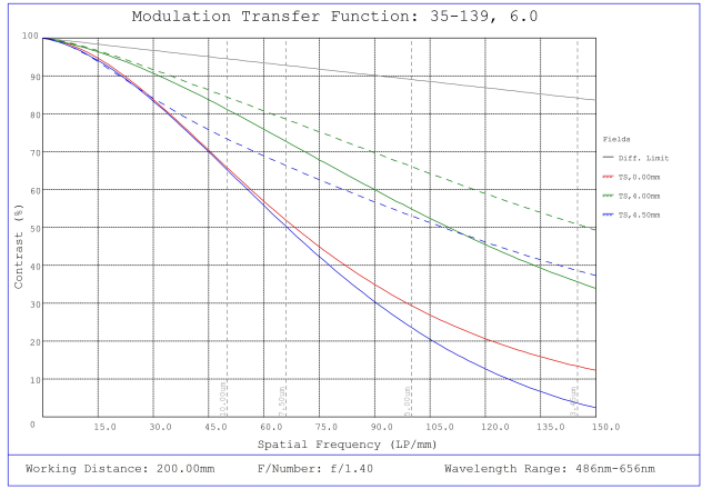
#35-139, 6mm, f/1.4 Cr Series Fixed Focal Length Lens, Modulated Transfer Function (MTF) Plot, 200mm Working Distance, f1.4
