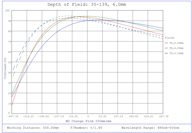
#35-139, 6mm, f/1.4 Cr Series Fixed Focal Length Lens, Depth of Field Plot, 500mm Working Distance, f1.4
