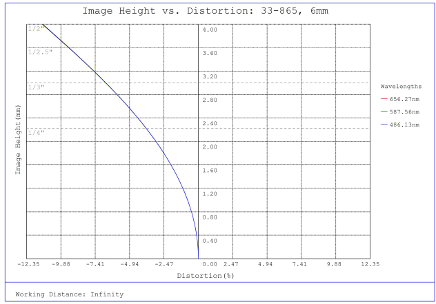
#33-865, 6mm, f/5.6 UCi Series Fixed Focal Length Lens, Distortion Plot
