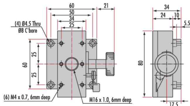
#55-026 - 60mm Travel, X-Axis Rack & Pinion Stage
