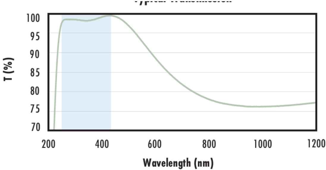
Fused Silica with UV-VIS Coating Typical Transmission
