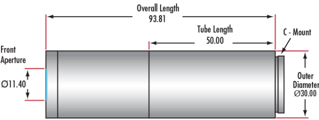
5X Compact Adjustable Objective (#88-353, #34-767)
