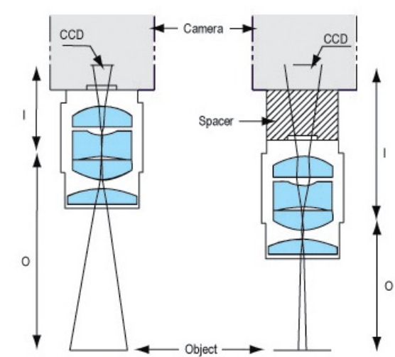
Using C-Mount Spacers in Electronic Imaging
