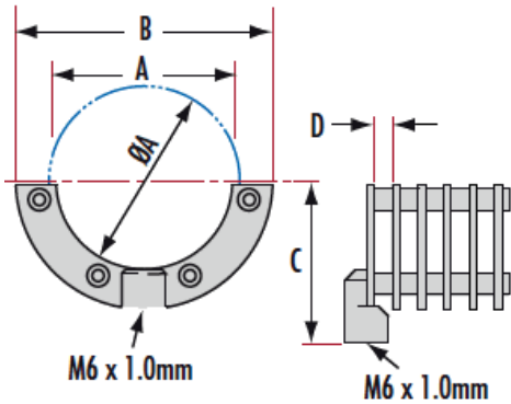
Mounting Cell
