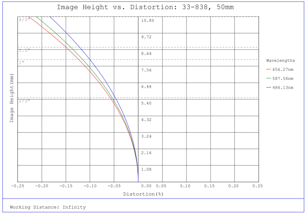
#33-838, 50mm f/5.6, HPI Series Fixed Focal Length Lens, Distortion Plot
