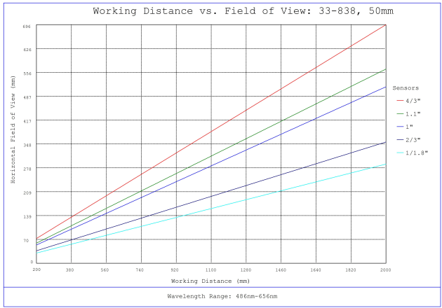
#33-838, 50mm f/5.6, HPI Series Fixed Focal Length Lens, Working Distance versus Field of View Plot
