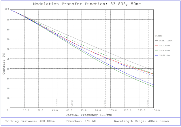
#33-838, 50mm f/5.6, HPi Series Fixed Focal Length Lens, Modulated Transfer Function (MTF) Plot, 400mm Working Distance, f5.6
