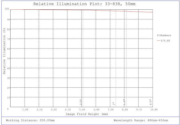
#33-838, 50mm f/5.6, HPI Series Fixed Focal Length Lens, Relative Illumination Plot
