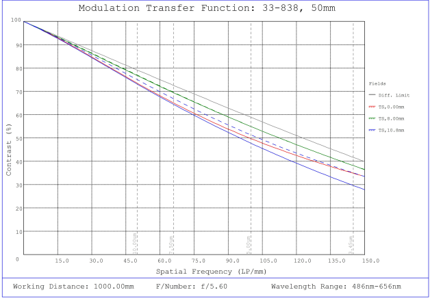
#33-838, 50mm f/5.6, HPi Series Fixed Focal Length Lens, Modulated Transfer Function (MTF) Plot, 1000mm Working Distance, f5.6
