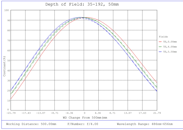
#35-192, 50mm, f/4.0 Cr Series Fixed Focal Length Lens, Depth of Field Plot, 500mm Working Distance, f4
