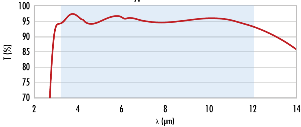
ZnSe with 3-12 microns AR Coating Typical Transmission
