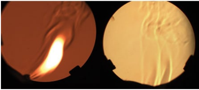
Flame Analysis using 6" Schlieren System
