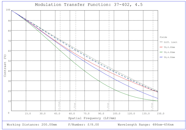
#37-402, 4.5mm, f/8 Cr Series Fixed Focal Length Lens, Modulated Transfer Function (MTF) Plot, 200mm Working Distance, f8
