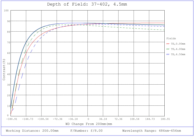
#37-402, 4.5mm, f/8 Cr Series Fixed Focal Length Lens, Depth of Field Plot, 200mm Working Distance, f8
