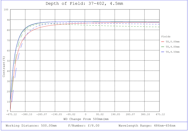
#37-402, 4.5mm, f/8 Cr Series Fixed Focal Length Lens, Depth of Field Plot, 500mm Working Distance, f8
