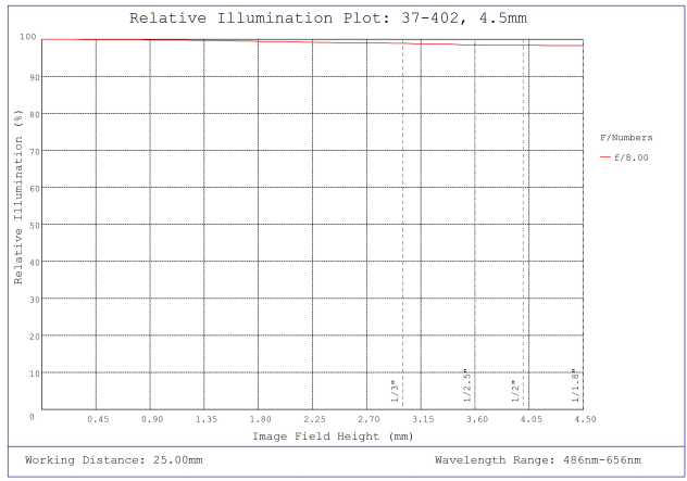
#37-402, 4.5mm, f/8 Cr Series Fixed Focal Length Lens, Relative Illumination Plot
