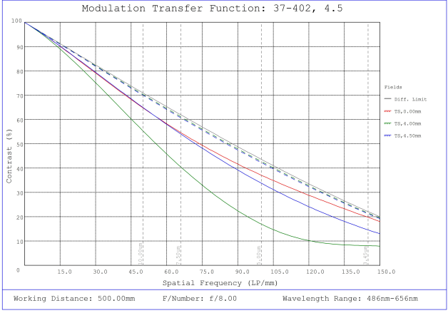
#37-402, 4.5mm, f/8 Cr Series Fixed Focal Length Lens, Modulated Transfer Function (MTF) Plot, 500mm Working Distance, f8
