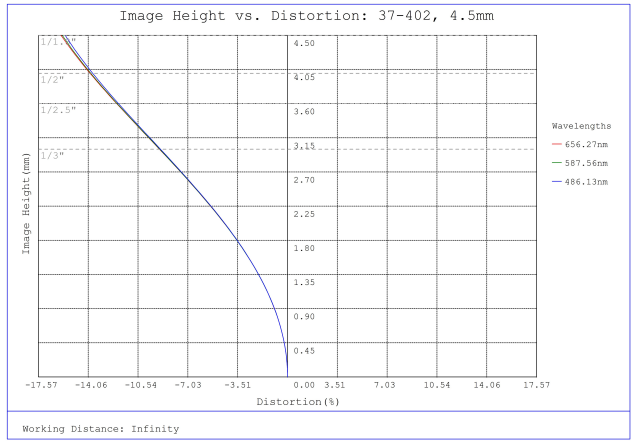
#37-402, 4.5mm, f/8 Cr Series Fixed Focal Length Lens, Distortion Plot
