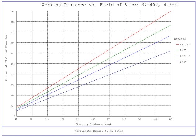
#37-402, 4.5mm, f/8 Cr Series Fixed Focal Length Lens, Working Distance versus Field of View Plot
