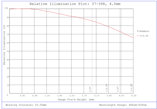
#37-398, 4.5mm, f/2 Cr Series Fixed Focal Length Lens, Relative Illumination Plot
