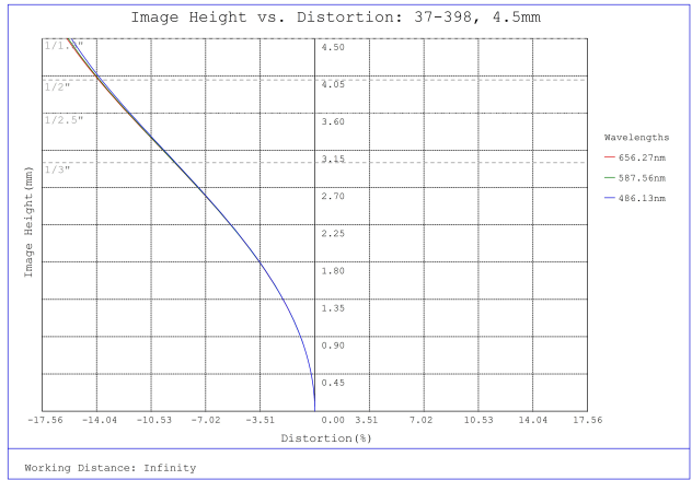
#37-398, 4.5mm, f/2 Cr Series Fixed Focal Length Lens, Distortion Plot
