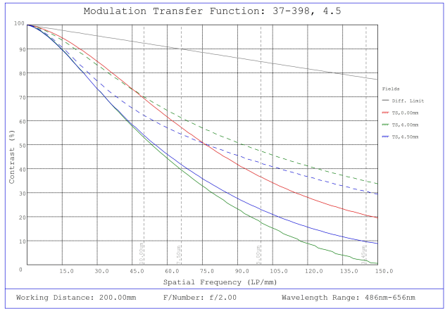
#37-398, 4.5mm, f/2 Cr Series Fixed Focal Length Lens, Modulated Transfer Function (MTF) Plot, 200mm Working Distance, f2
