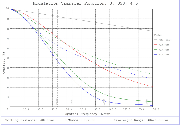
#37-398, 4.5mm, f/2 Cr Series Fixed Focal Length Lens, Modulated Transfer Function (MTF) Plot, 500mm Working Distance, f2
