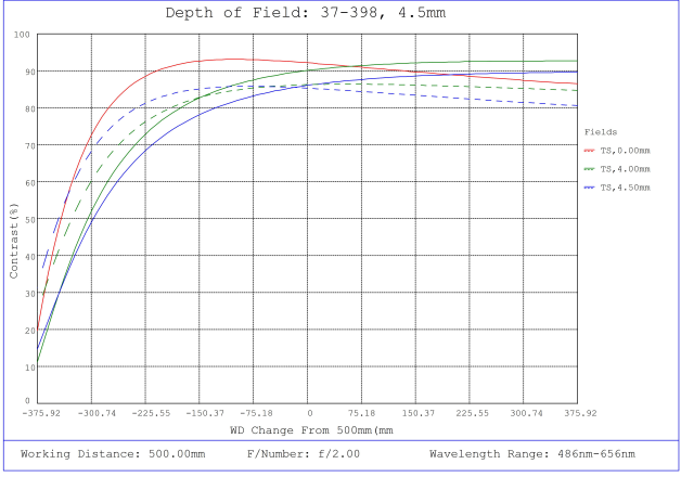
#37-398, 4.5mm, f/2 Cr Series Fixed Focal Length Lens, Depth of Field Plot, 500mm Working Distance, f2
