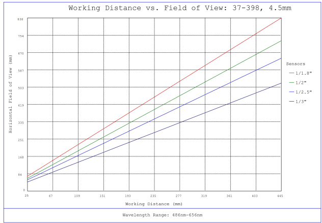
#37-398, 4.5mm, f/2 Cr Series Fixed Focal Length Lens, Working Distance versus Field of View Plot
