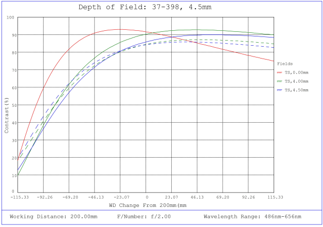
#37-398, 4.5mm, f/2 Cr Series Fixed Focal Length Lens, Depth of Field Plot, 200mm Working Distance, f2
