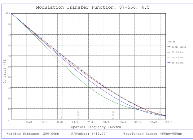
#87-556, 4.5mm, f/11 Ci Series Fixed Focal Length Lens, Modulated Transfer Function (MTF) Plot, 200mm Working Distance, f11
