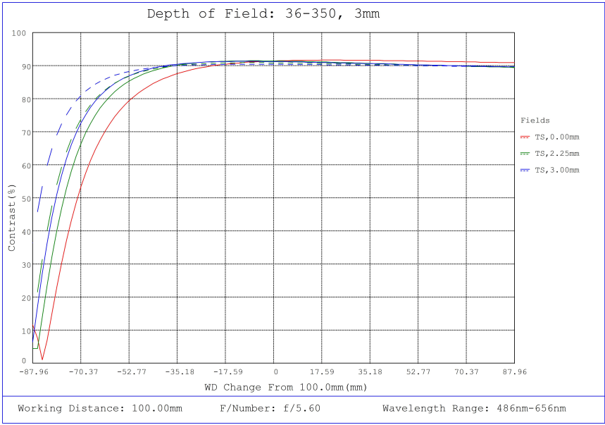
#36-350, 3mm FL f/5.6, Rugged Blue Series M12 Lens, Depth of Field Plot, 100mm Working Distance, f5.6
