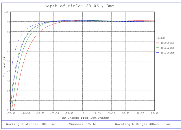
#20-061, 3mm FL f/5.6 IR-Cut Rugged Blue Series M12 Lens, Depth of Field Plot, 100mm Working Distance, f5.6
