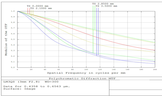
3mm FL, f/2.8, Low Distortion M12 Lens, MTF Plot
