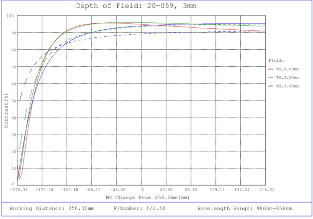
#20-059, 3mm FL f/2.5 IR-Cut Rugged Blue Series M12 Lens, Depth of Field Plot, 250mm Working Distance, f2.5
