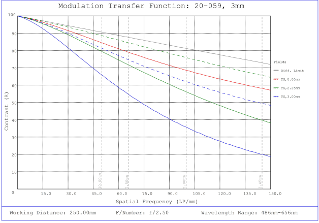
#20-059, 3mm FL f/2.5 IR-Cut Rugged Blue Series M12 Lens, Modulated Transfer Function (MTF) Plot, 250mm Working Distance, f2.5
