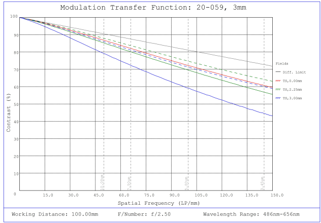
#20-059, 3mm FL f/2.5 IR-Cut Rugged Blue Series M12 Lens, Modulated Transfer Function (MTF) Plot, 100mm Working Distance, f2.5
