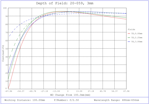
#20-059, 3mm FL f/2.5 IR-Cut Rugged Blue Series M12 Lens, Depth of Field Plot, 100mm Working Distance, f2.5
