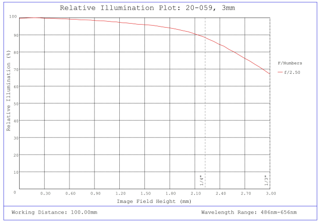
#20-059, 3mm FL f/2.5 IR-Cut Rugged Blue Series M12 Lens, Relative Illumination Plot
