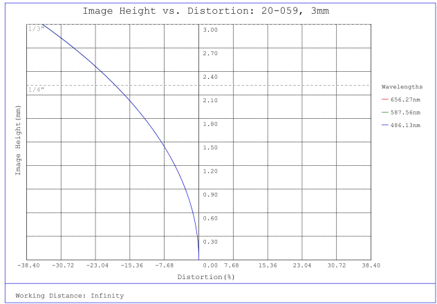
#20-059, 3mm FL f/2.5 IR-Cut Rugged Blue Series M12 Lens, Distortion Plot
