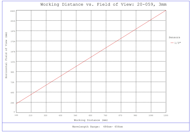
#20-059, 3mm FL f/2.5 IR-Cut Rugged Blue Series M12 Lens, Working Distance versus Field of View Plot
