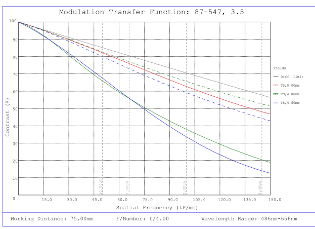
#87-547, 3.5mm, f/4 Ci Series Fixed Focal Length Lens, Modulated Transfer Function (MTF) Plot, 75mm Working Distance, f4
