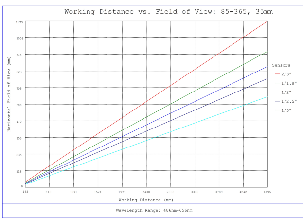
#85-365, 35mm, f/4 Ci Series Fixed Focal Length Lens, Working Distance versus Field of View Plot
