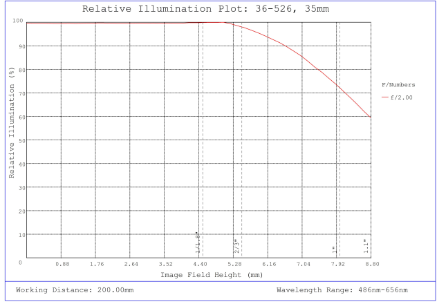
#36-526, 35mm f/2.0, HPr Series Fixed Focal Length Lens, Relative Illumination Plot
