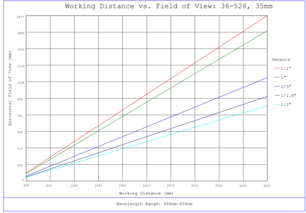
#36-526, 35mm f/2.0, HPr Series Fixed Focal Length Lens, Working Distance versus Field of View Plot
