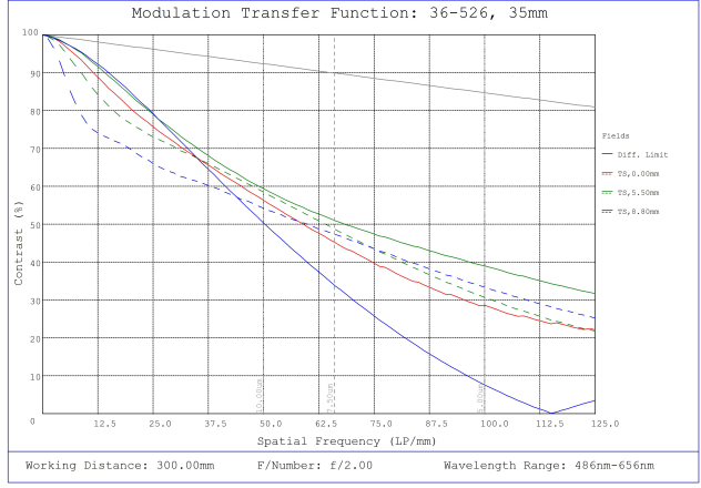
#36-526, 35mm f/2.0, HPr Series Fixed Focal Length Lens, Modulated Transfer Function (MTF) Plot, 300mm Working Distance, f2
