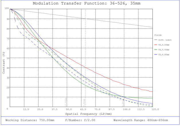
#36-526, 35mm f/2.0, HPr Series Fixed Focal Length Lens, Modulated Transfer Function (MTF) Plot, 750mm Working Distance, f2
