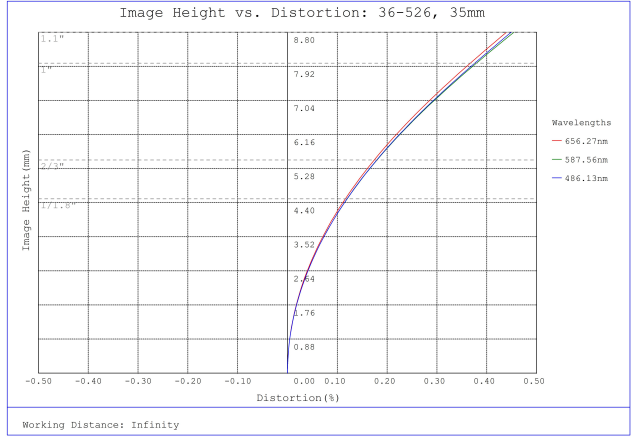
#36-526, 35mm f/2.0, HPr Series Fixed Focal Length Lens, Distortion Plot
