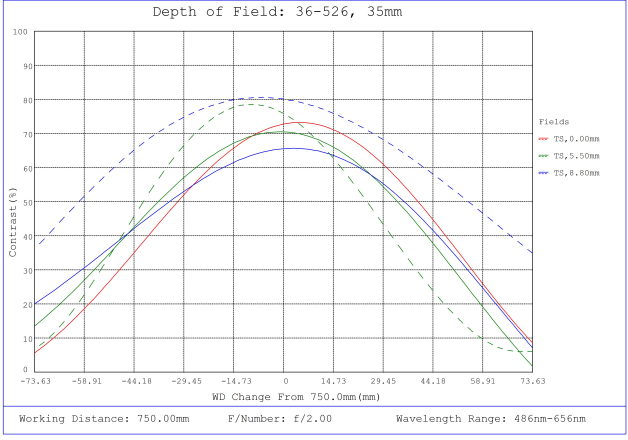
#36-526, 35mm f/2.0, HPr Series Fixed Focal Length Lens, Depth of Field Plot, 750mm Working Distance, f2
