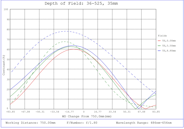
#36-525, 35mm f/1.8, HPr Series Fixed Focal Length Lens, Depth of Field Plot, 750mm Working Distance, f1.8
