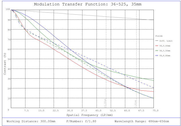
#36-525, 35mm f/1.8, HPr Series Fixed Focal Length Lens, Modulated Transfer Function (MTF) Plot, 300mm Working Distance, f1.8
