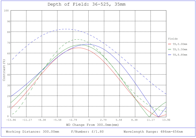
#36-525, 35mm f/1.8, HPr Series Fixed Focal Length Lens, Depth of Field Plot, 300mm Working Distance, f1.8
