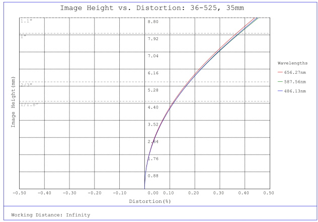
#36-525, 35mm f/1.8, HPr Series Fixed Focal Length Lens, Distortion Plot
