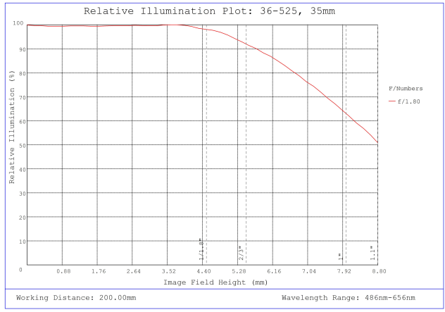
#36-525, 35mm f/1.8, HPr Series Fixed Focal Length Lens, Relative Illumination Plot
