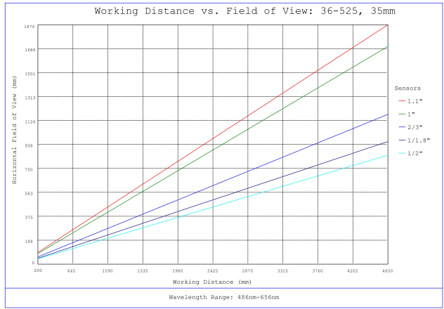
#36-525, 35mm f/1.8, HPr Series Fixed Focal Length Lens, Working Distance versus Field of View Plot
