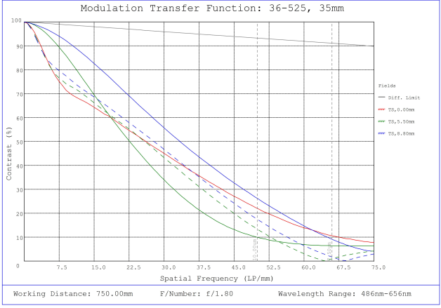
#36-525, 35mm f/1.8, HPr Series Fixed Focal Length Lens, Modulated Transfer Function (MTF) Plot, 750mm Working Distance, f1.8
