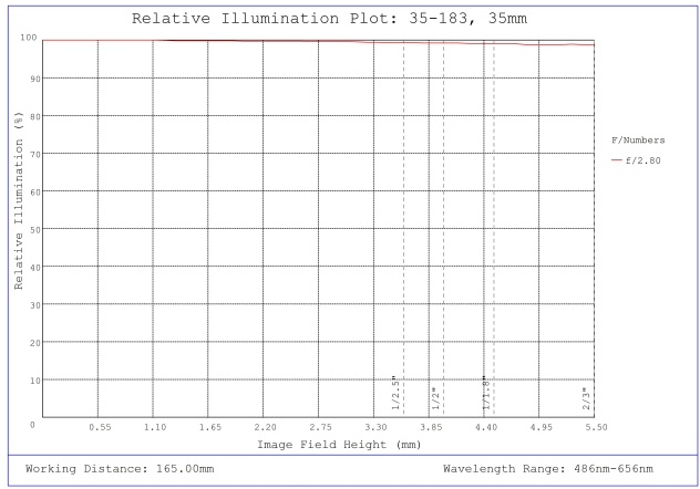
#35-183, 35mm, f/2.8 Cr Series Fixed Focal Length Lens, Relative Illumination Plot
