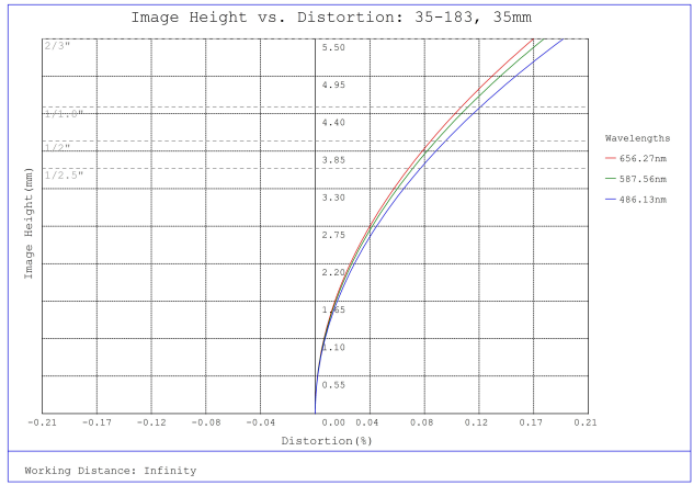
#35-183, 35mm, f/2.8 Cr Series Fixed Focal Length Lens, Distortion Plot
