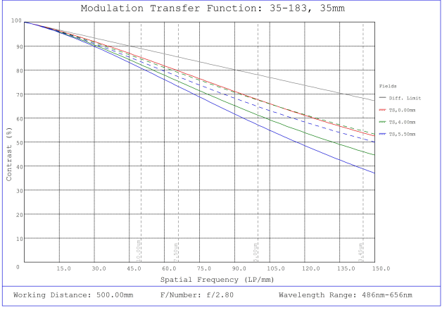
#35-183, 35mm, f/2.8 Cr Series Fixed Focal Length Lens, Modulated Transfer Function (MTF) Plot, 500mm Working Distance, f2.8
