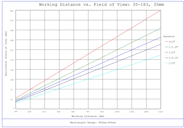
#35-183, 35mm, f/2.8 Cr Series Fixed Focal Length Lens, Working Distance versus Field of View Plot
