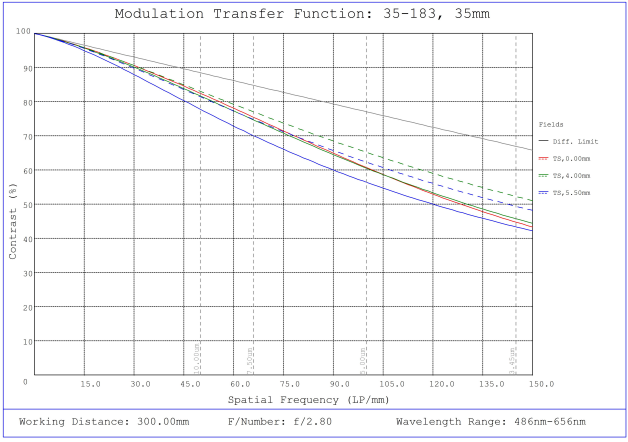
#35-183, 35mm, f/2.8 Cr Series Fixed Focal Length Lens, Modulated Transfer Function (MTF) Plot, 300mm Working Distance, f2.8
