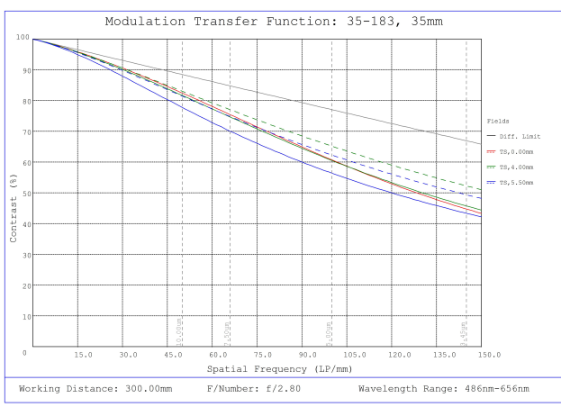
#35-183, 35mm, f/2.8 Cr Series Fixed Focal Length Lens, Modulated Transfer Function (MTF) Plot, 300mm Working Distance, f2.8
