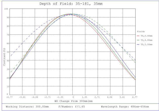
#35-181, 35mm, f/1.65 Cr Series Fixed Focal Length Lens, Depth of Field Plot, 300mm Working Distance, f1.6
