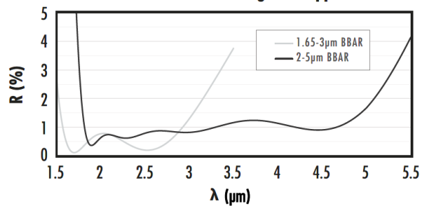
Infrared AR Coated Sapphire Windows 1mm Thickness
