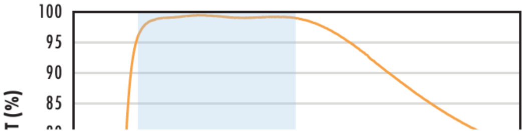
N-BK7 with VIS-EXT Coating Typical Transmission
