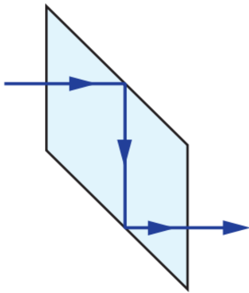
Rhomboid Prism Ray Path
